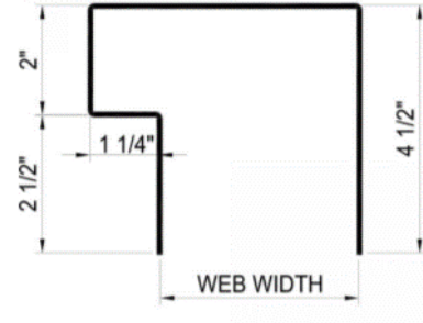
#15 2 HR, 3" total deflection
