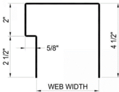
#11 1HR, 3" total deflection
